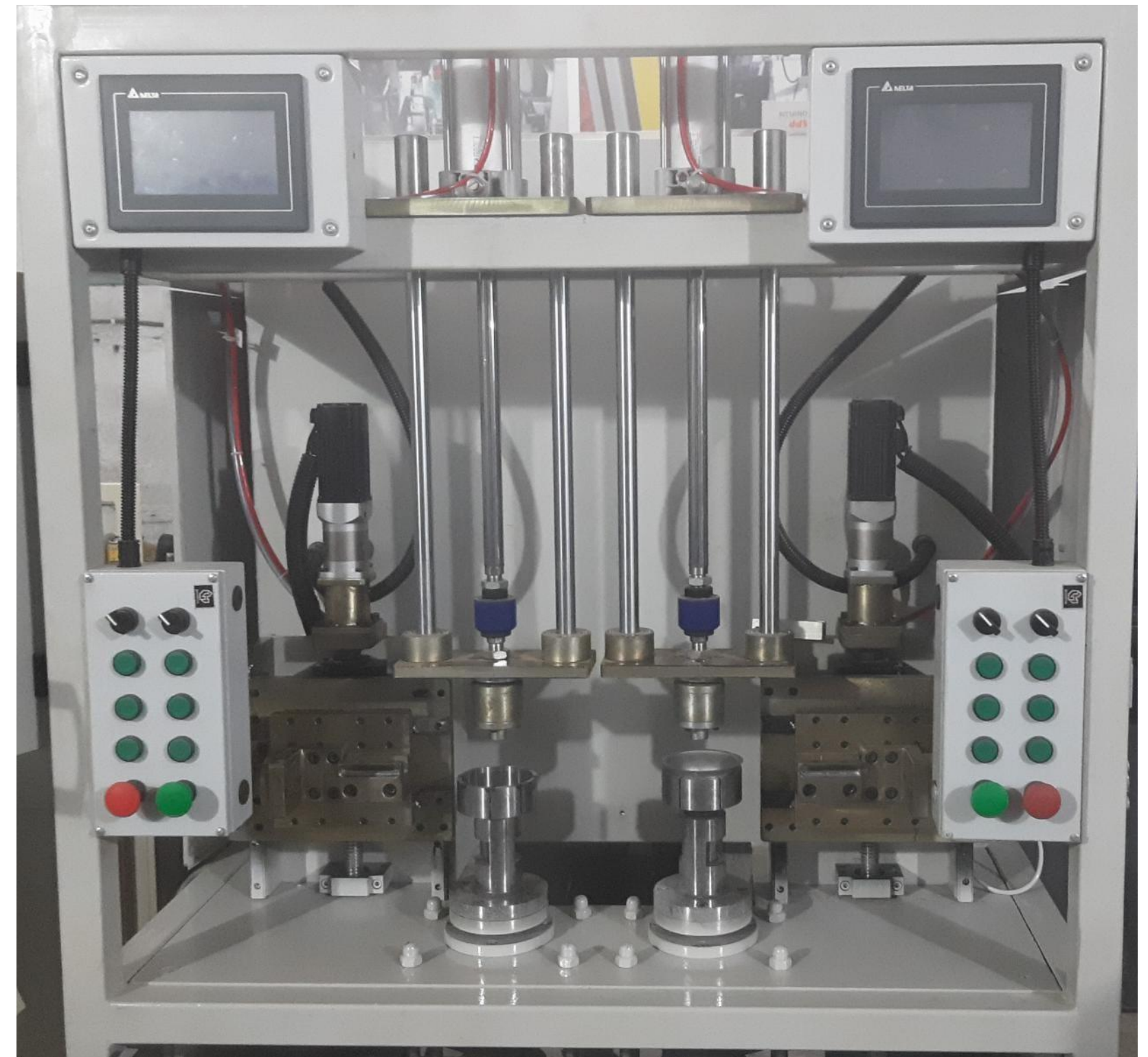
Trimming SPM on Bottom cover of water bottle
